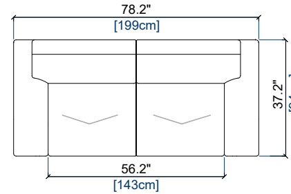
CANAPÉ 2.5 PLACES 2.5-SEAT SOFA SOFA 2,5 PLAZAS
